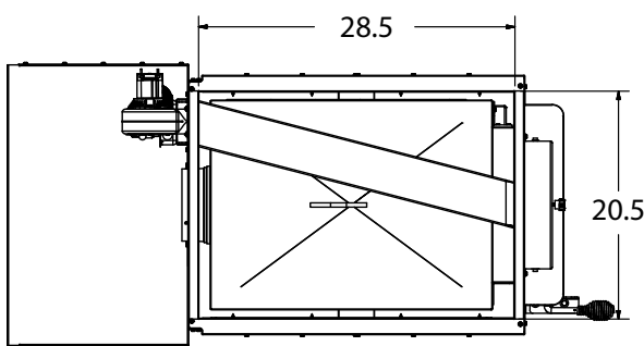
Supply Air Duct Work Outlet Size
